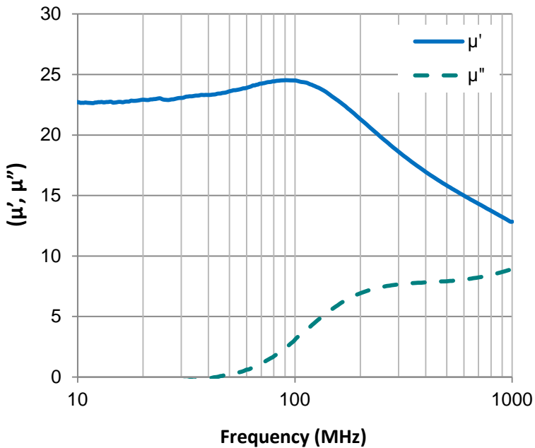
Measured Complex Permeability
