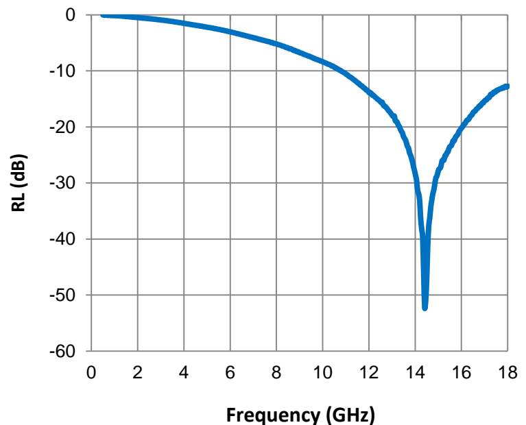
Reflection Loss
