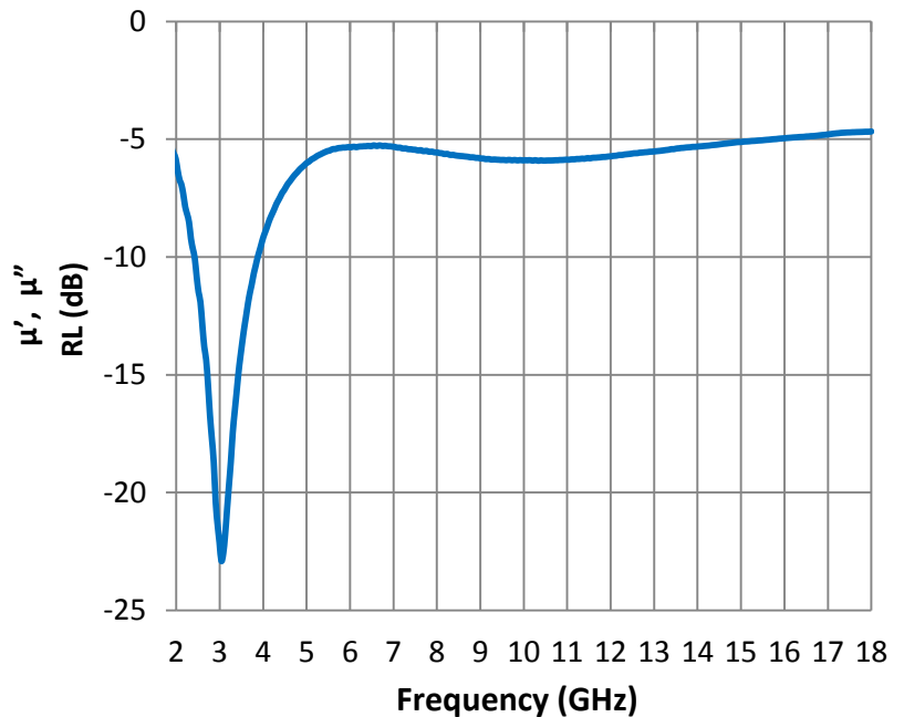
Reflection Loss
