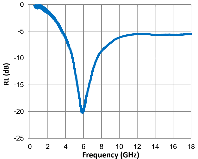
Reflection Loss
