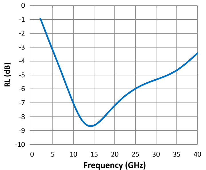
Reflection Loss
