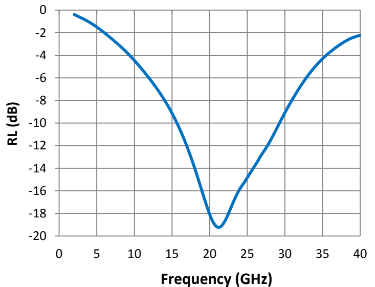
Reflection Loss
