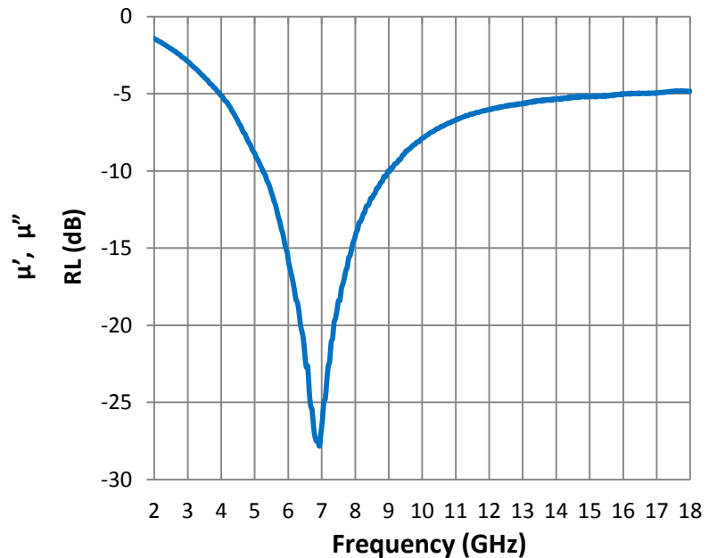
Reflection Loss
