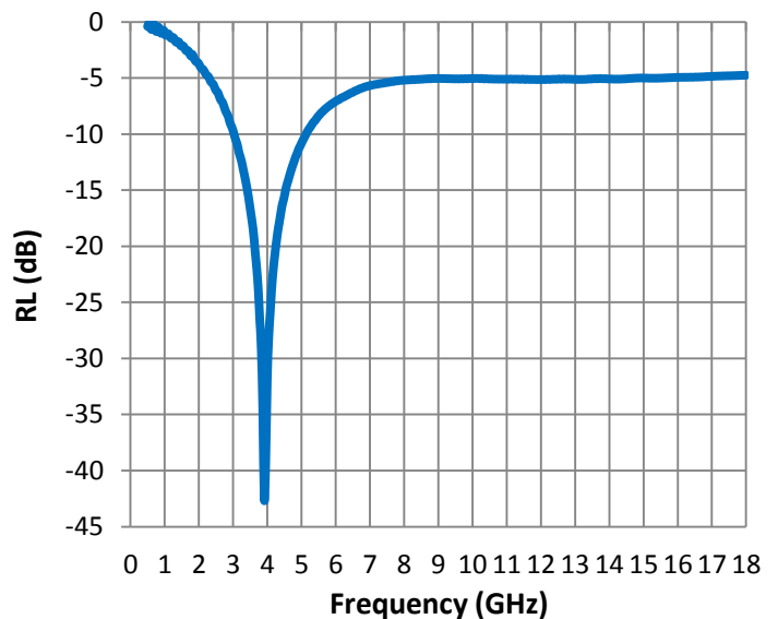
Reflection Loss
