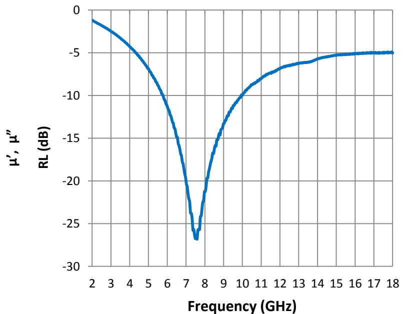
Reflection Loss
