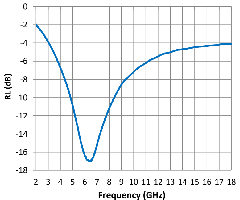
Reflection Loss
