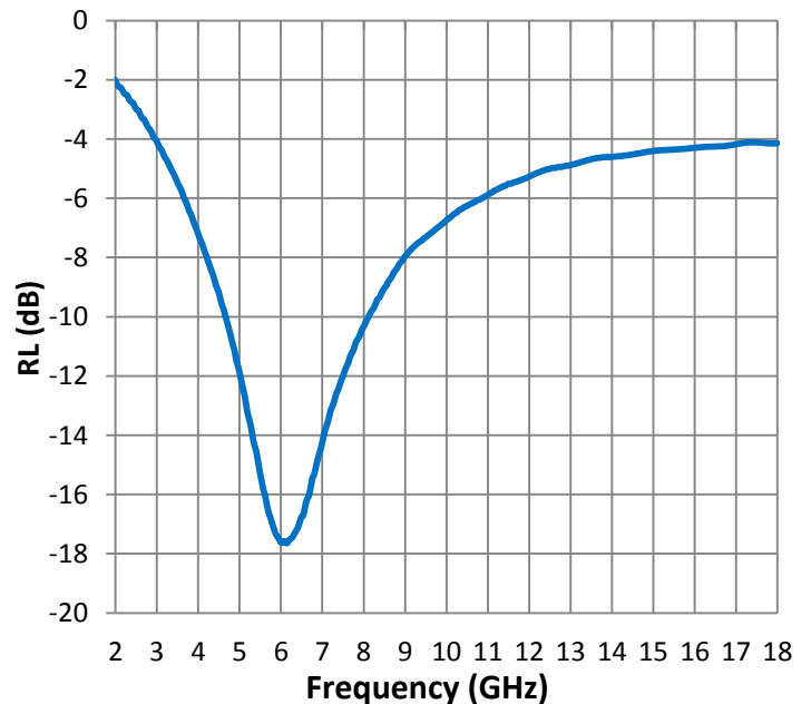
Reflection Loss
