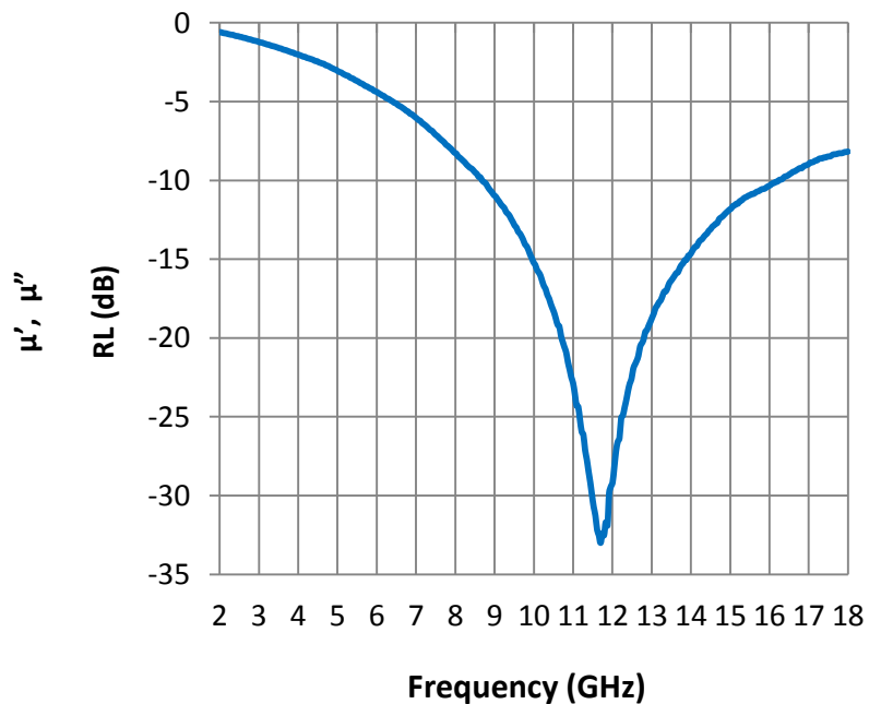
Reflection Loss
