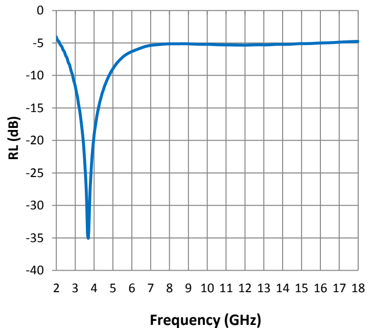
Reflection Loss
