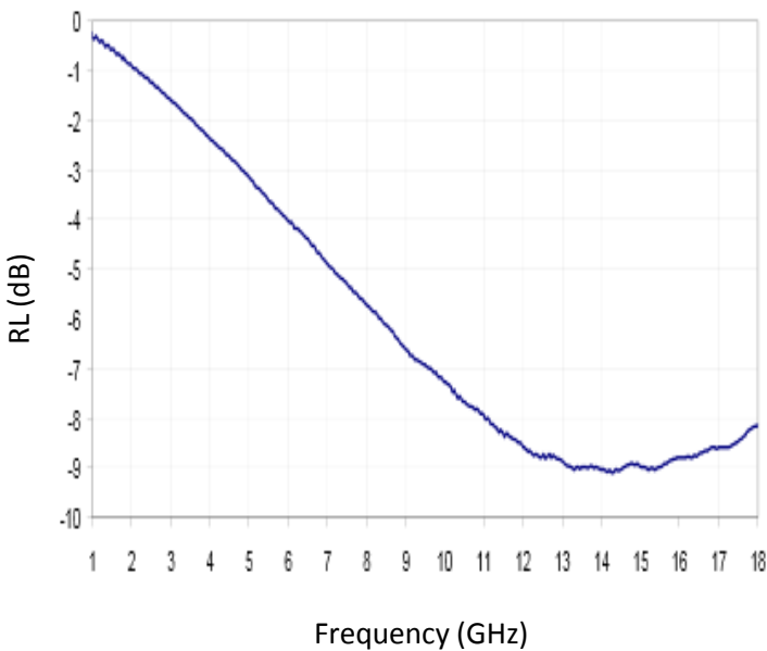
Reflection Loss
