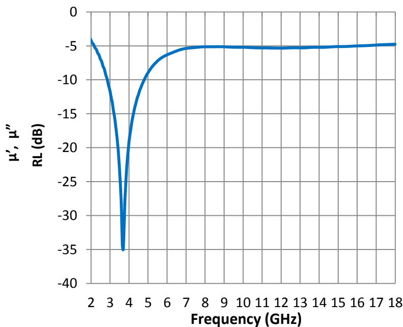
Reflection Loss
