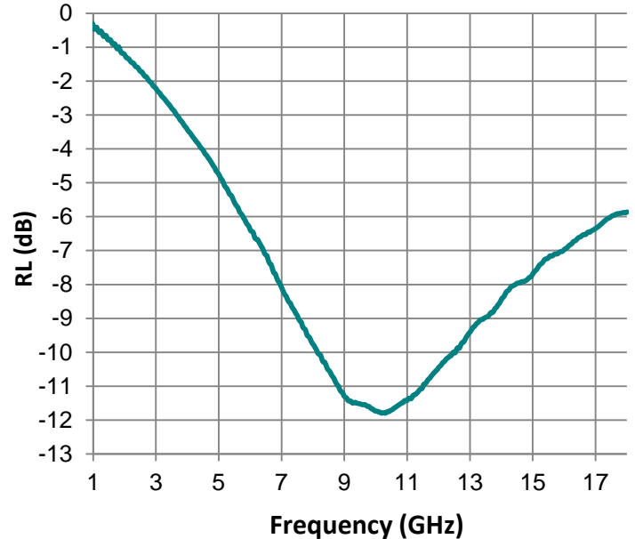
Reflection Loss
