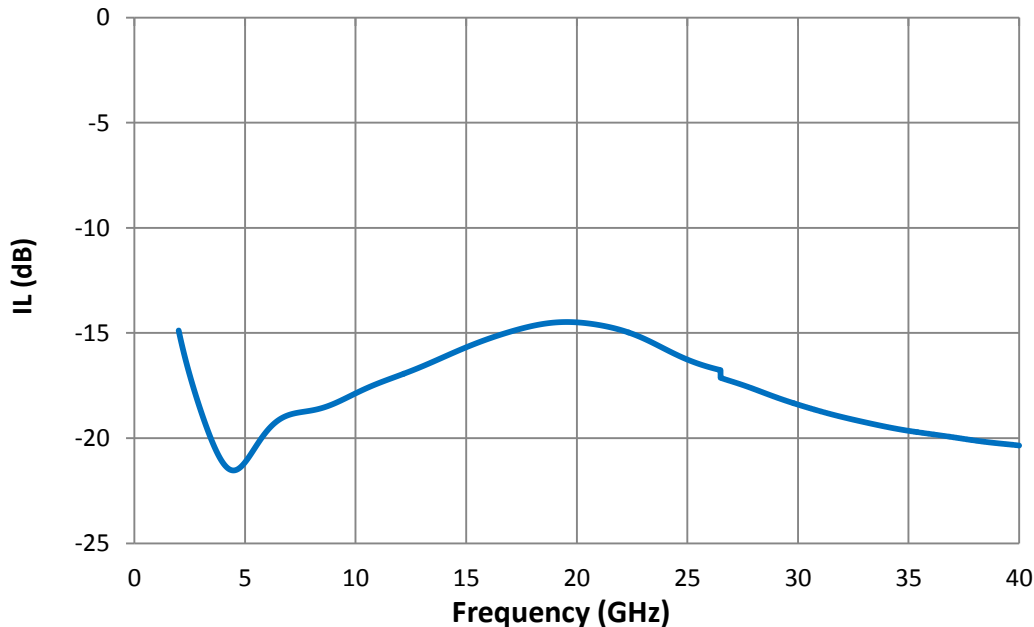
Insertion Loss
