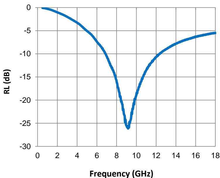
Reflection Loss
