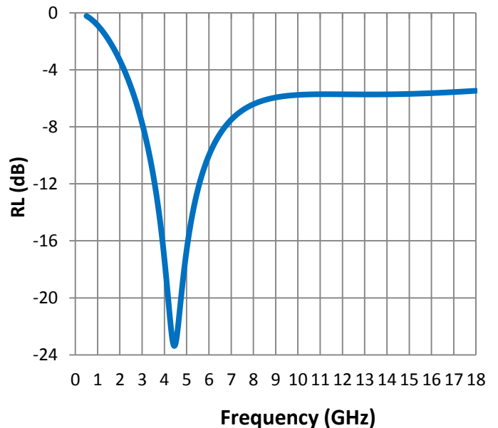
Reflection Loss
