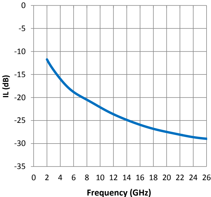
Insertion Loss
