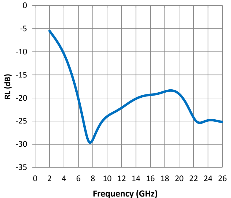
Reflection Loss
