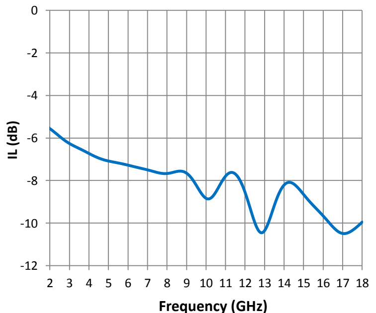
Insertion Loss
