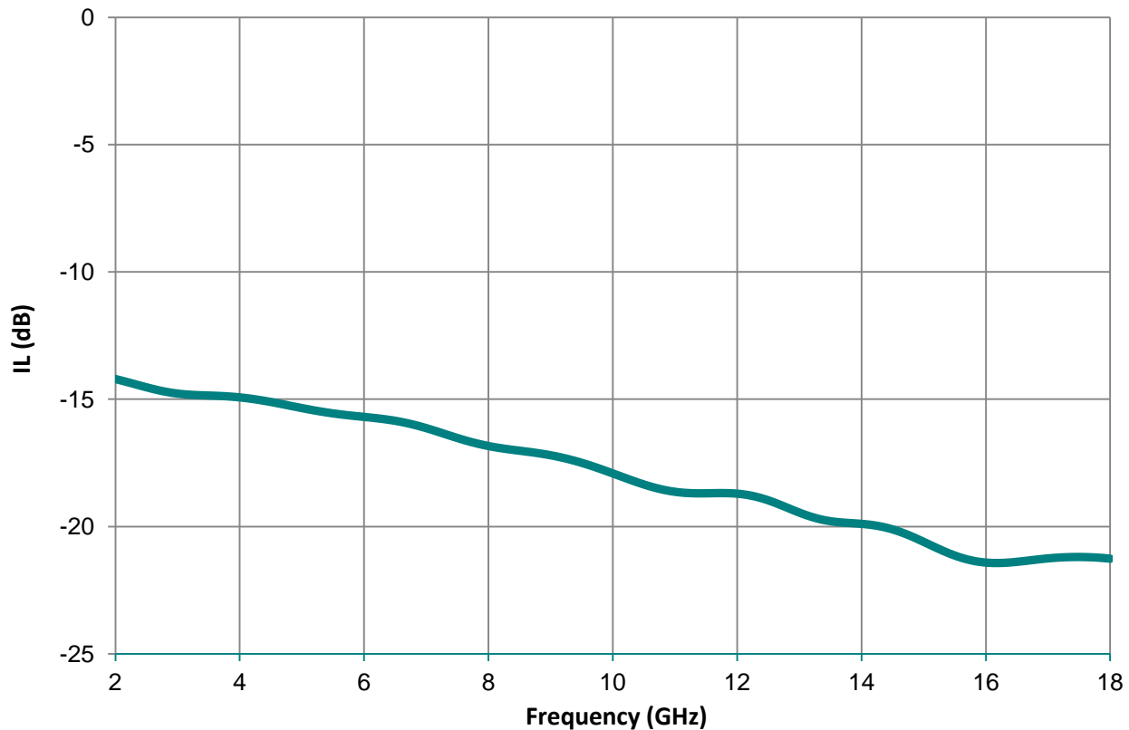
Insertion Loss of LS-10055-40
