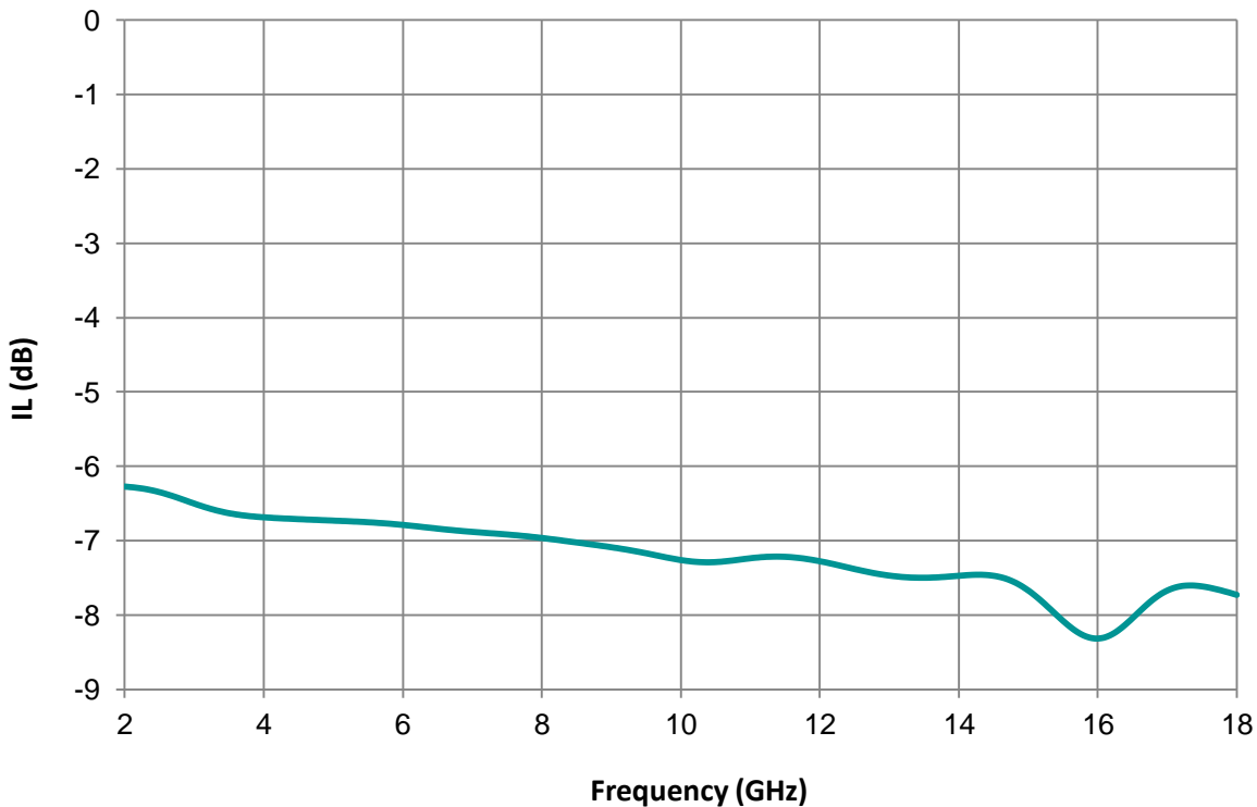
Insertion Loss of LS-10246
