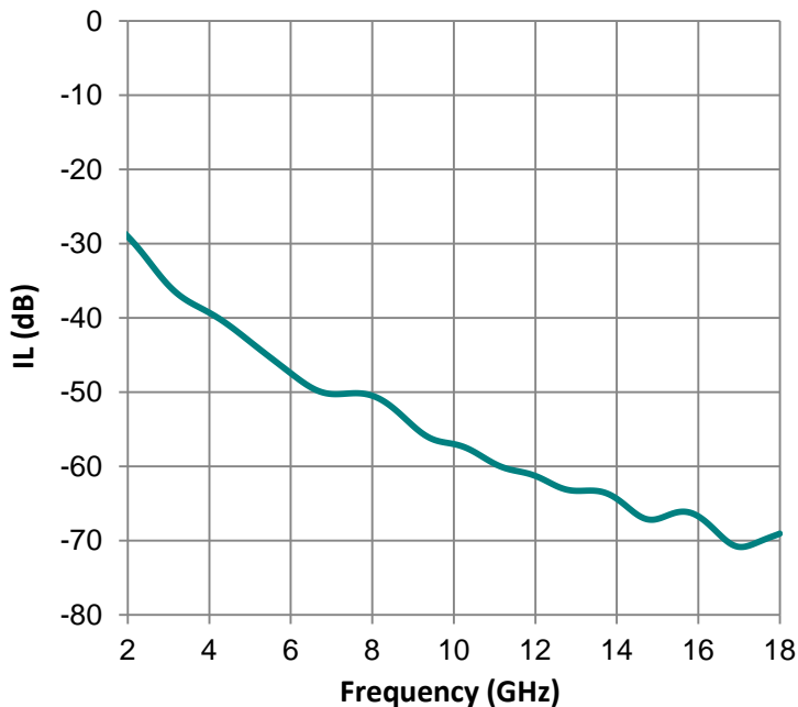
Insertion Loss of LS-10426
