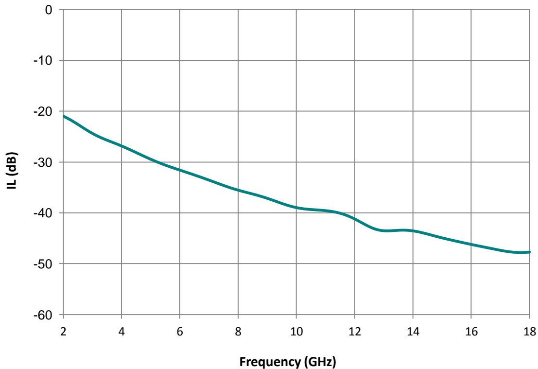
Insertion Loss of LS-10569
