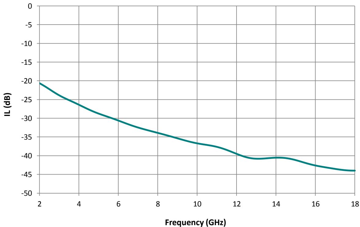
Insertion Loss of LS-10640
