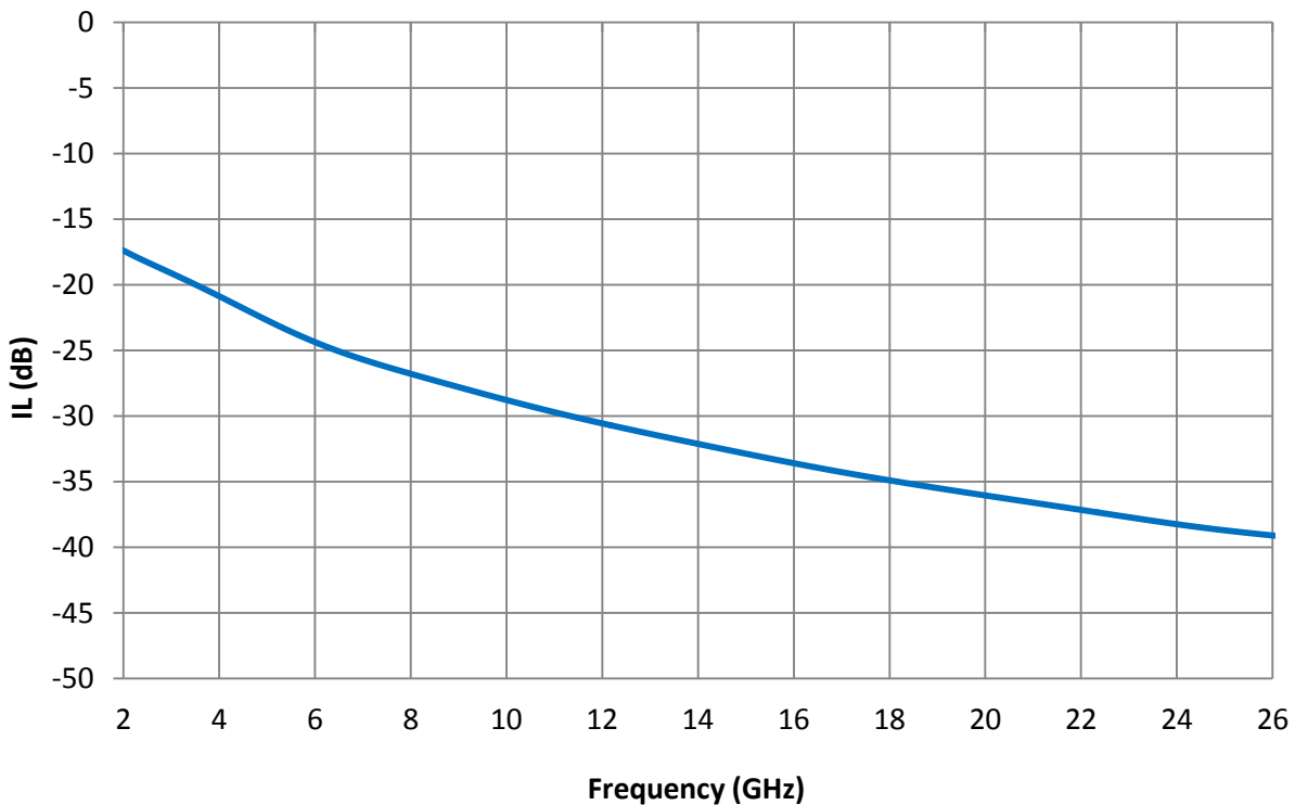
Insertion Loss
