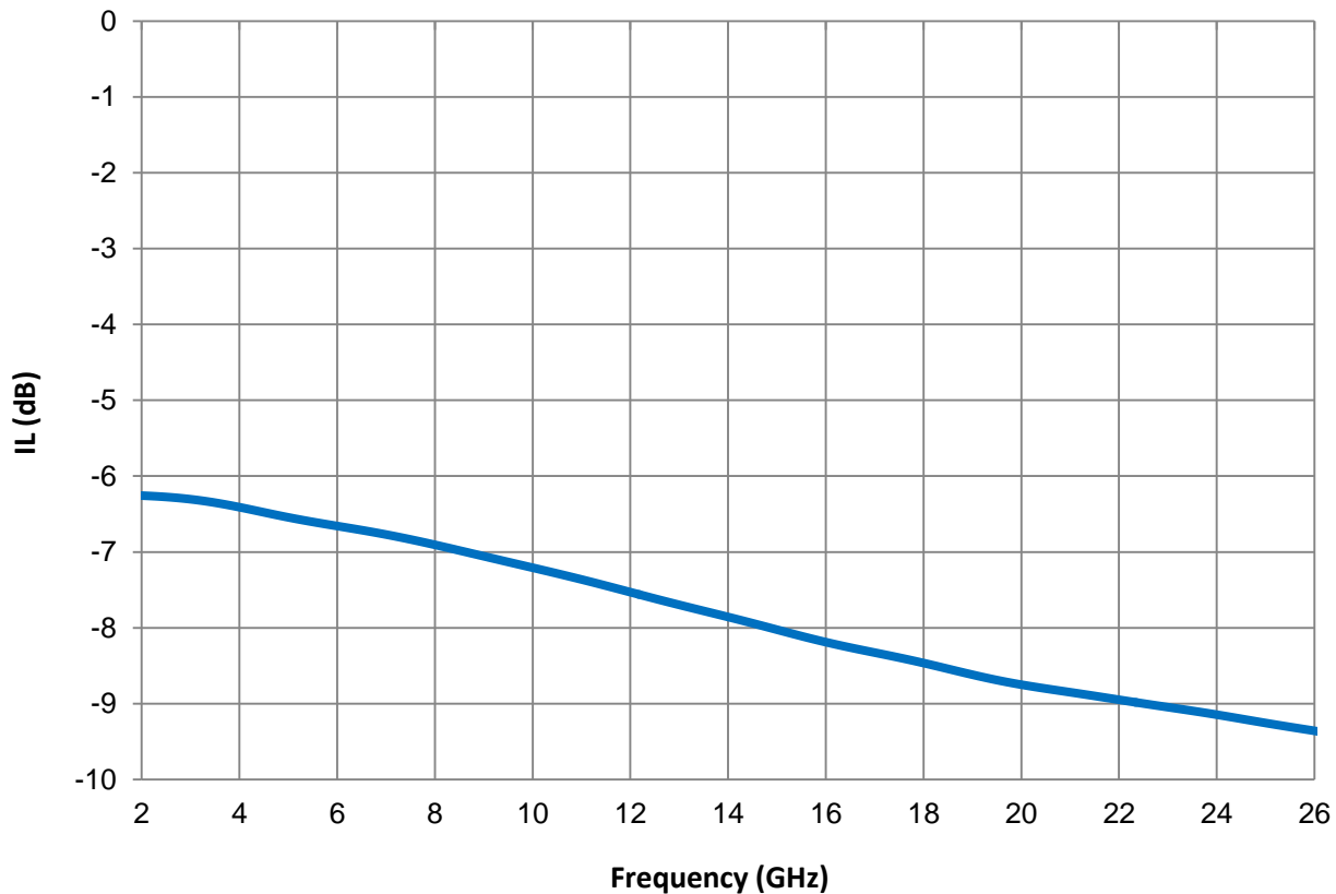
Insertion Loss
