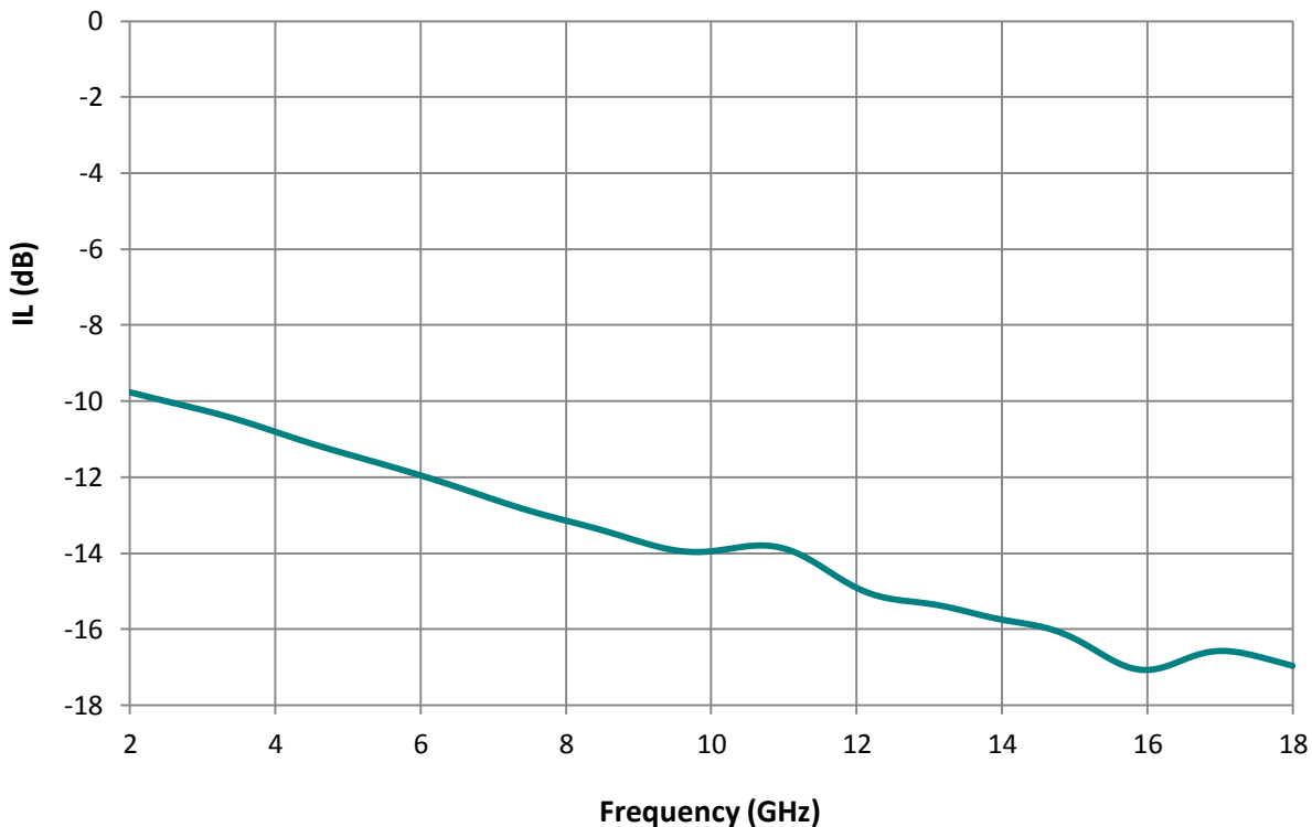
Insertion Loss of LS-11059
