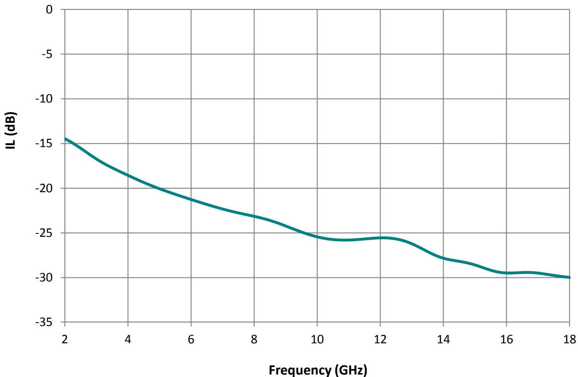
Insertion Loss of LS-11073
