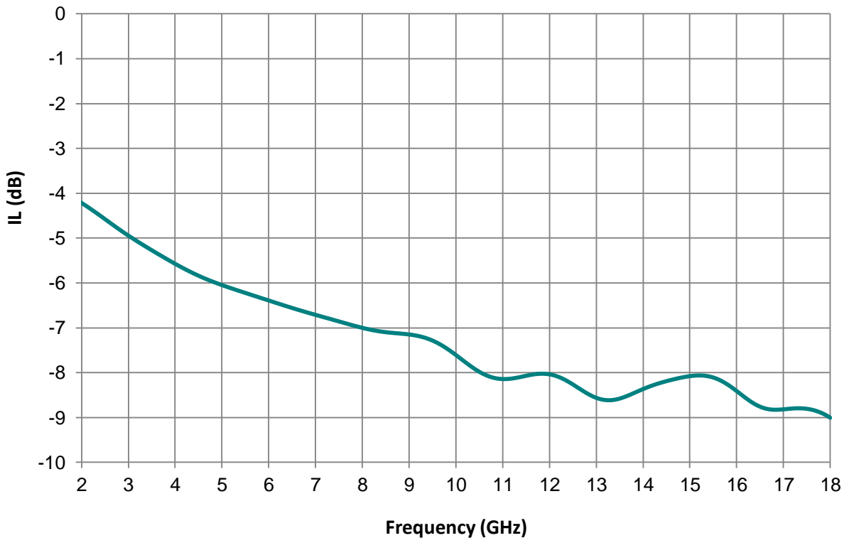
Insertion Loss of LS-12792
