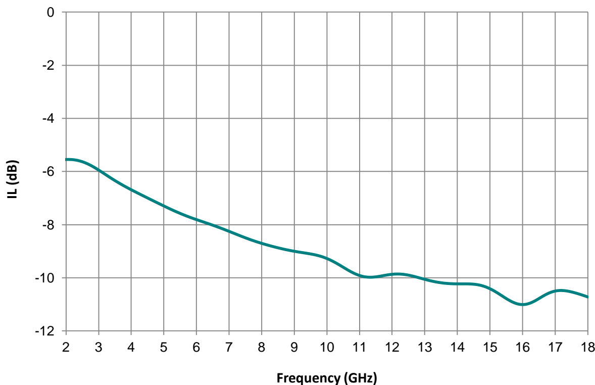
Insertion Loss of LS-55174
