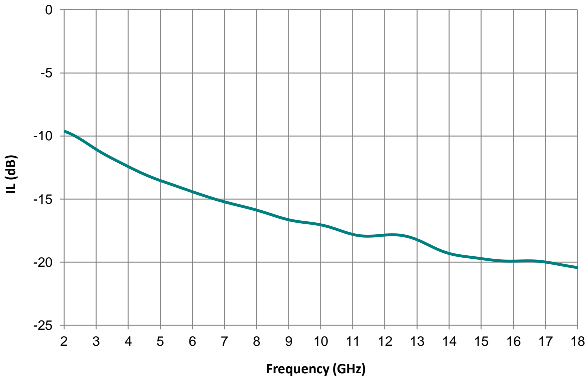
Insertion Loss of LS-55217
