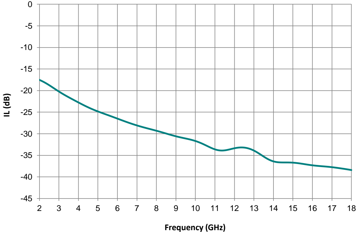
Insertion Loss of LS-55219
