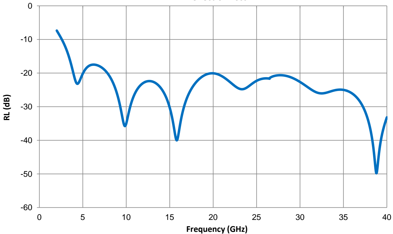
Reflection Loss
