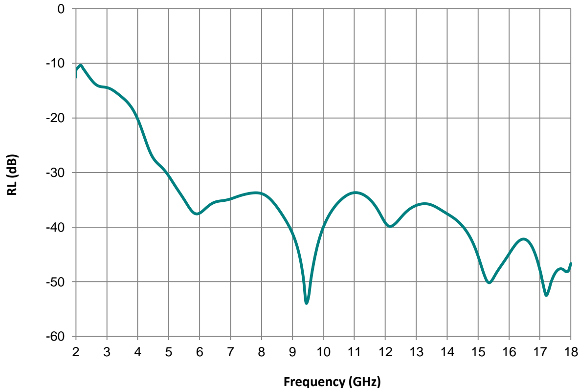
Reflection Loss of RC-10398
