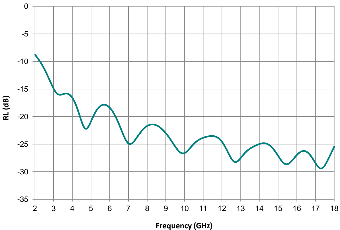
Reflection Loss of RT-10448
