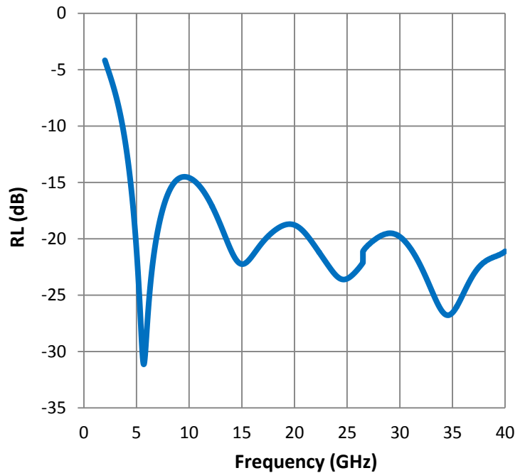
Reflection Loss
