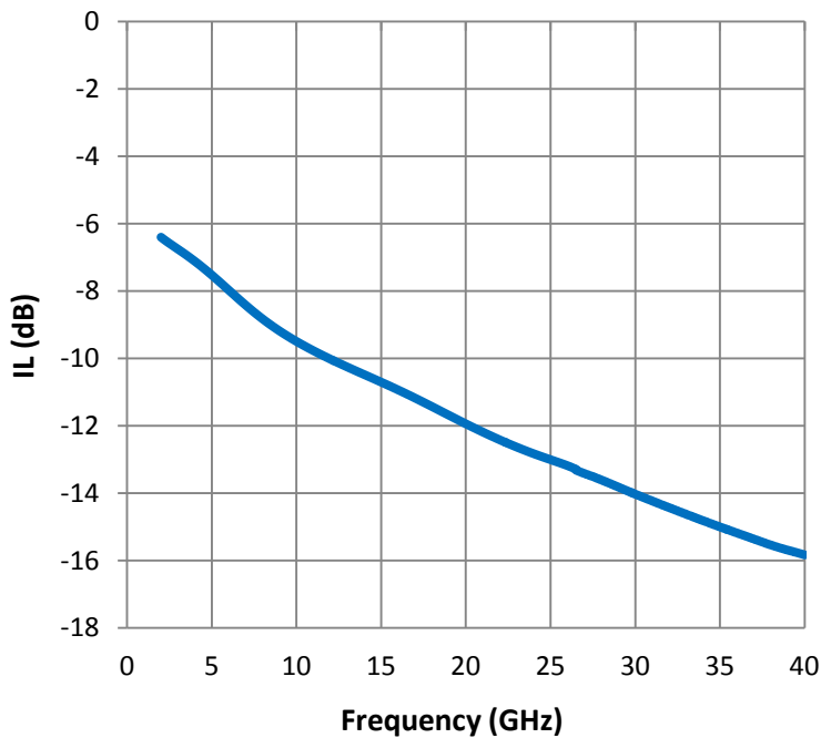
Insertion Loss
