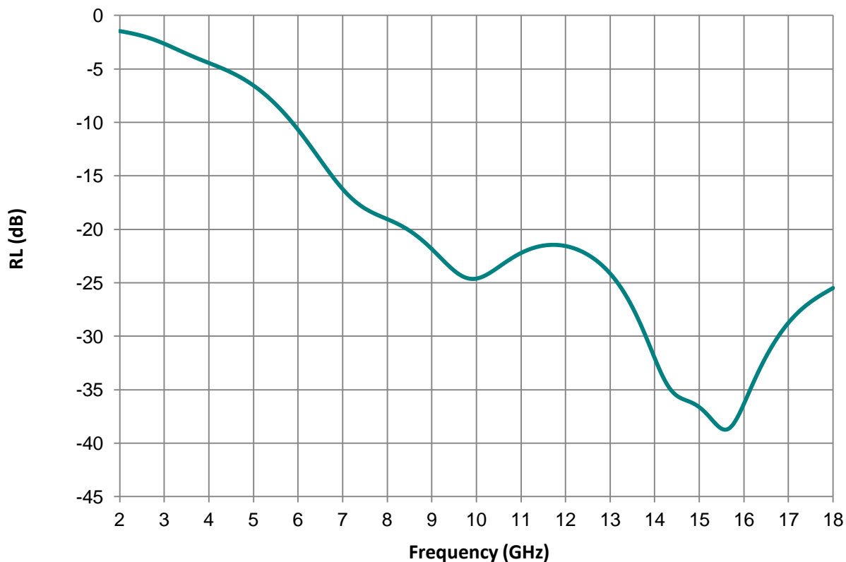
Reflection Loss of RT-13445-1
