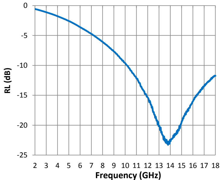
Reflection Loss
