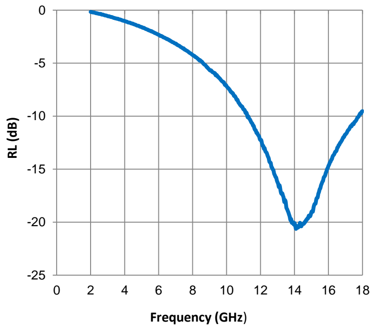
Reflection Loss
