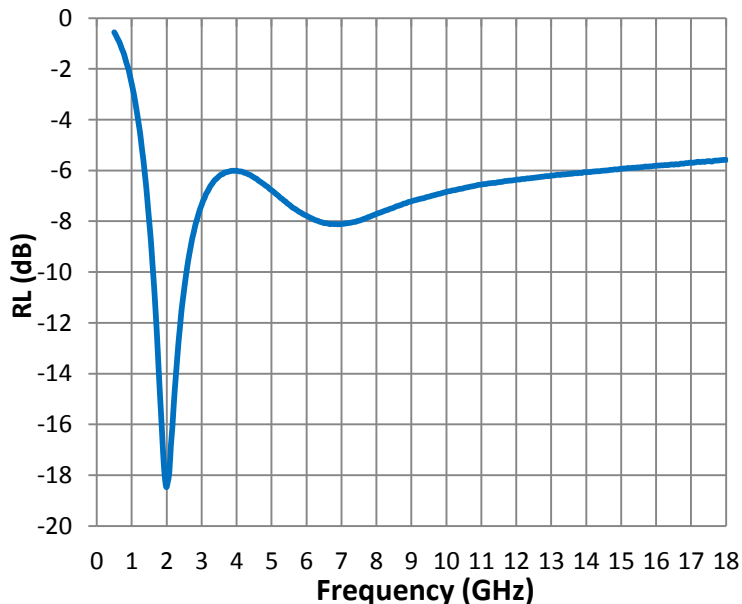
Reflection Loss
