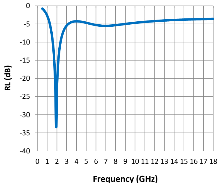
Reflection Loss
