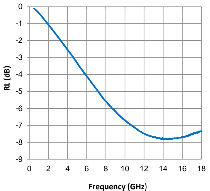
Reflection Loss
