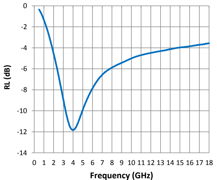
Reflection Loss
