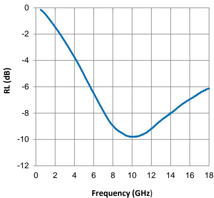
Reflection Loss
