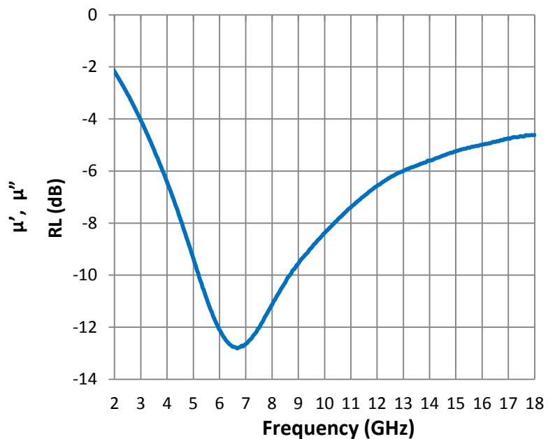
Reflection Loss
