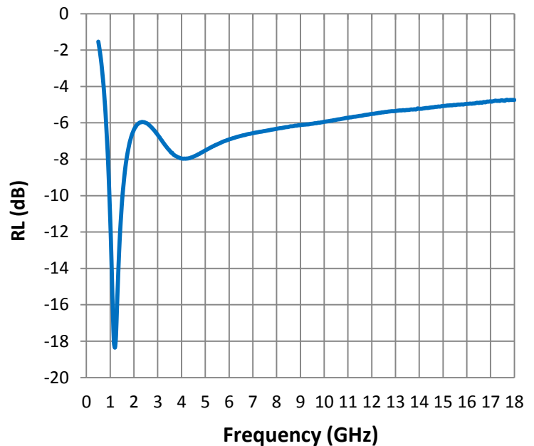
Reflection Loss
