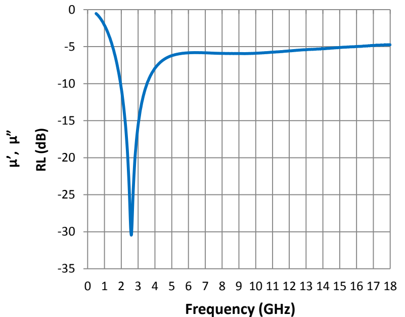
Reflection Loss
