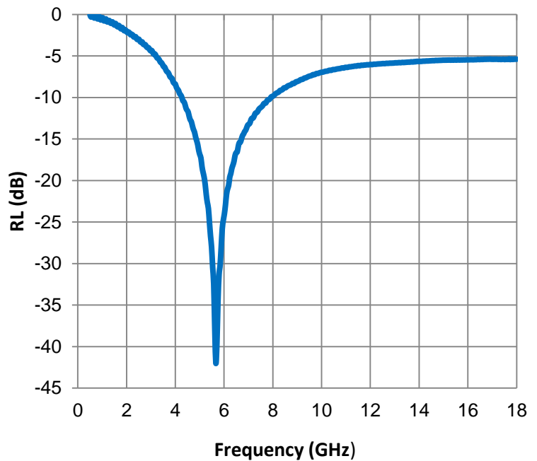
Reflection Loss
